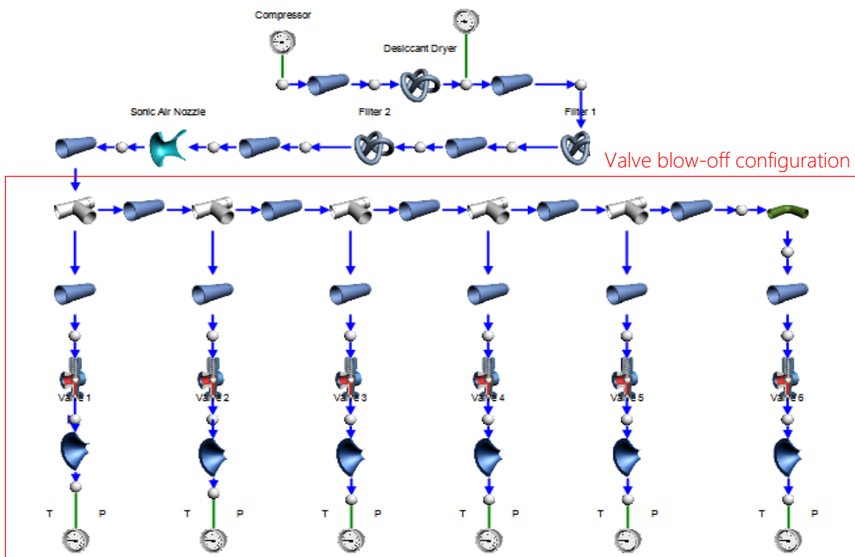
Figure 1: Flownex® Blow-off configuration.
