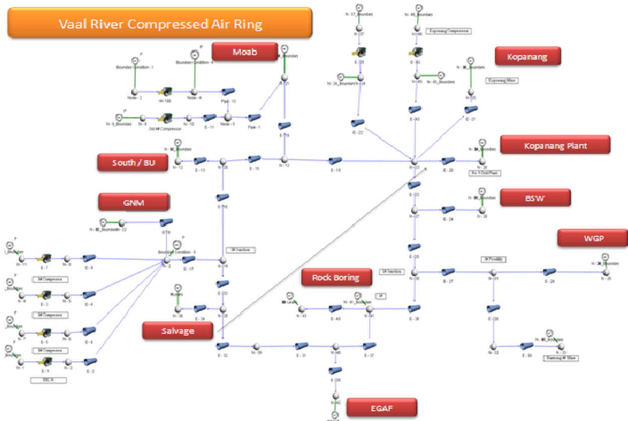
Figure 1: Flownex simulation of the compressed air network.
