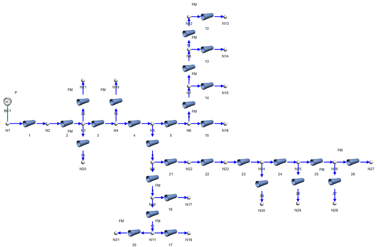
Figure 2: Flownex network.
