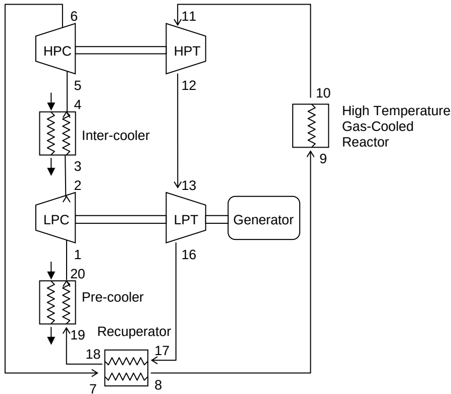
Figure 1: Two-shaft closed inter-cooled recuperated Brayton cycle.
