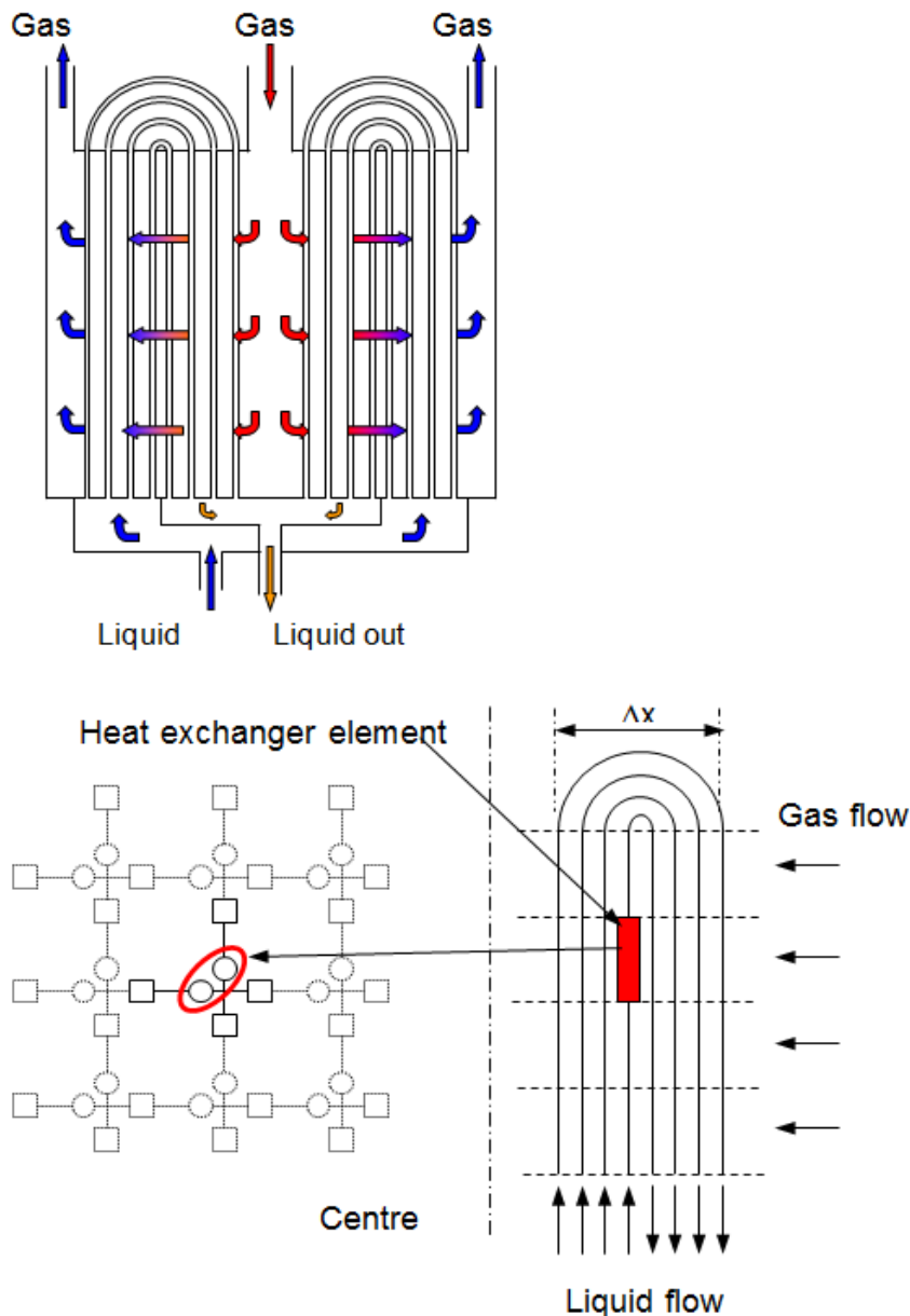
Figure 3: Discretization of the pre-cooler.
