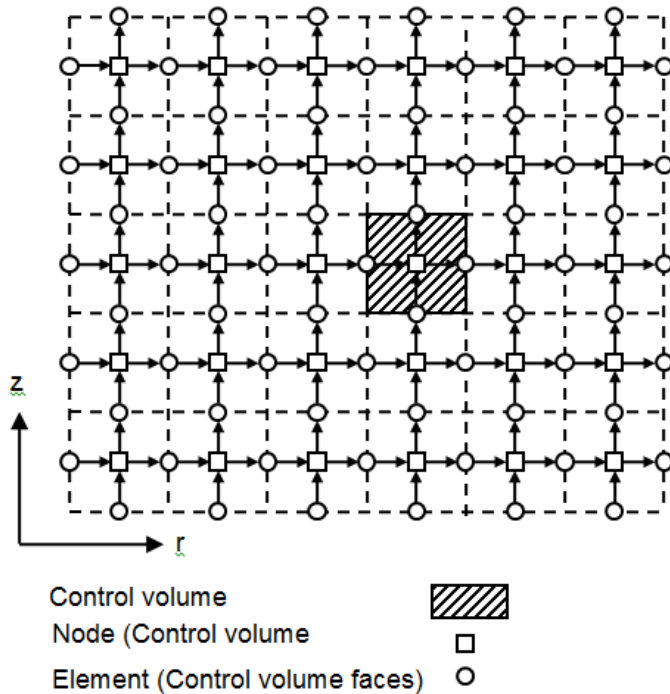
Figure 5: Flownex network representation of staggered CFD grid.
