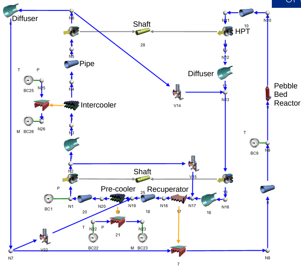
Figure 2: Flownex network of the direct two-shaft closed inter-cooled recuperated Brayton cycle PBMR power plant.
