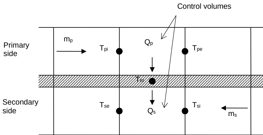
Figure 4: Discretization of counter/parallel flow heat exchanger.
