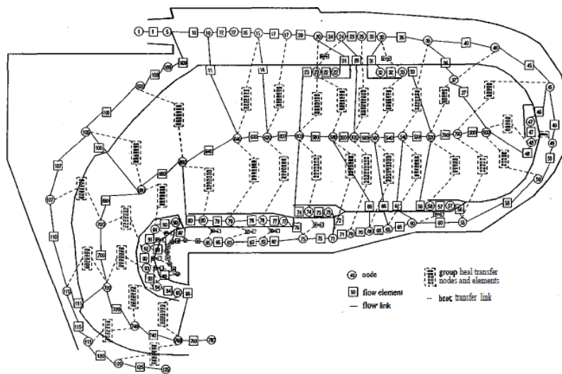
Figure 2: Network diagram for reverse flow combustor
