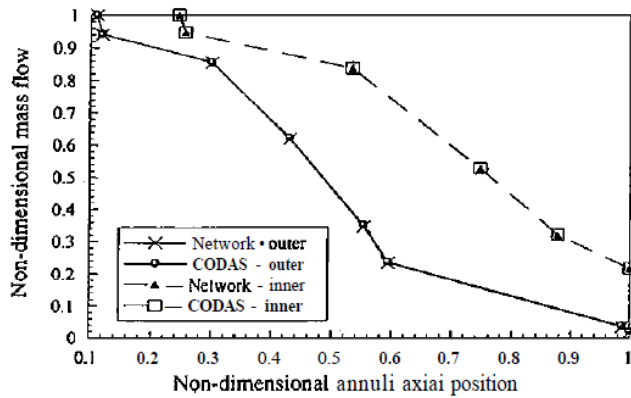
Figure 3: Annular combustor 1: Comparison between network method- and CODAS results for non-dimensional mass flow vs. non-dimensional annuli axial position.
