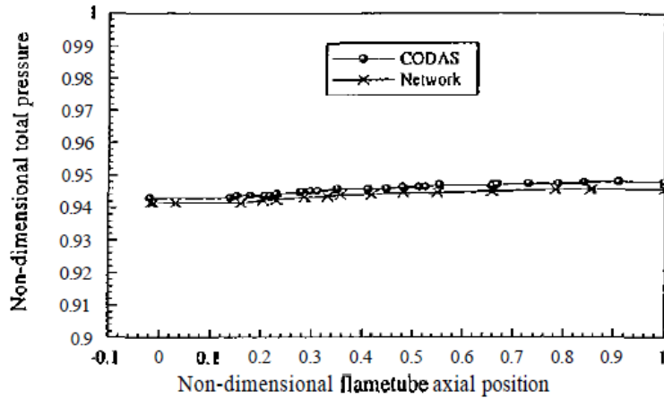
Figure 6: Annular combustor 2: Comparison between network method- and CODAS results for non-dimensional total pressure vs. non-dimensional flame tube axial position.
