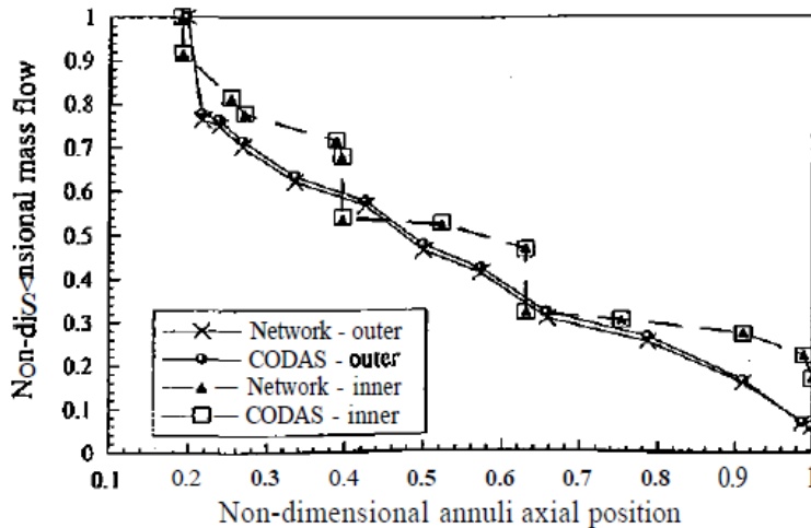
Figure 5: Annular combustor 2: Comparison between network method- and CODAS results for non-dimensional mass flow vs. non-dimensional annuli axial position.
