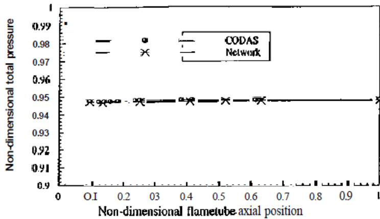
Figure 4: Annular combustor 1: Comparison between network method- and CODAS results for non-dimensional total pressure vs. non-dimensional flame tube axial position.
