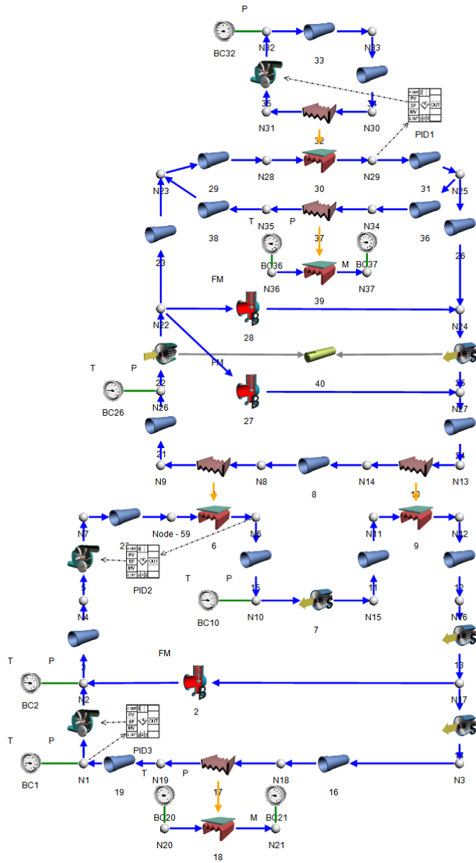
Figure 2: Flownex model of the Combined Cycle High Temperature Reactor Gas-Cooled Power Plant.
