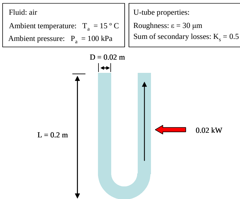
Figure 1: Schematic layout of a U-tube in which air is flowing due to natural convection.
