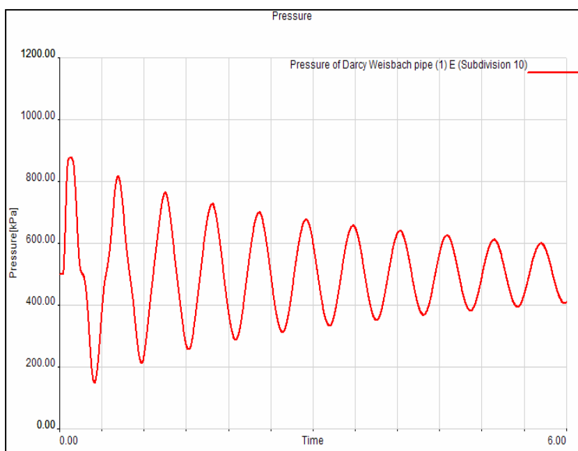
Figure 4: Water hammer simulation results.
