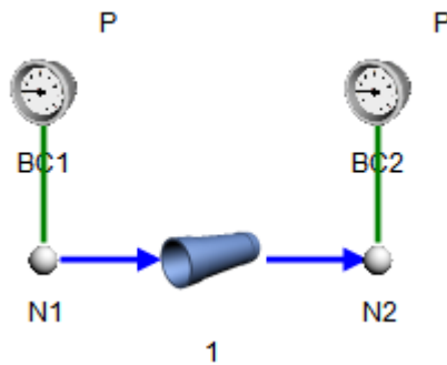
Figure 2: Flownex network.
