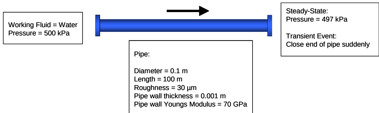
Figure 1: Schematic layout of a pipe in which water is flowing, and a valve is suddenly closed at the outlet end.
