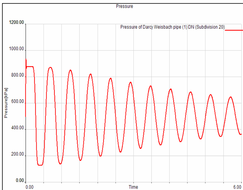
Figure 3: Water hammer simulation results.
