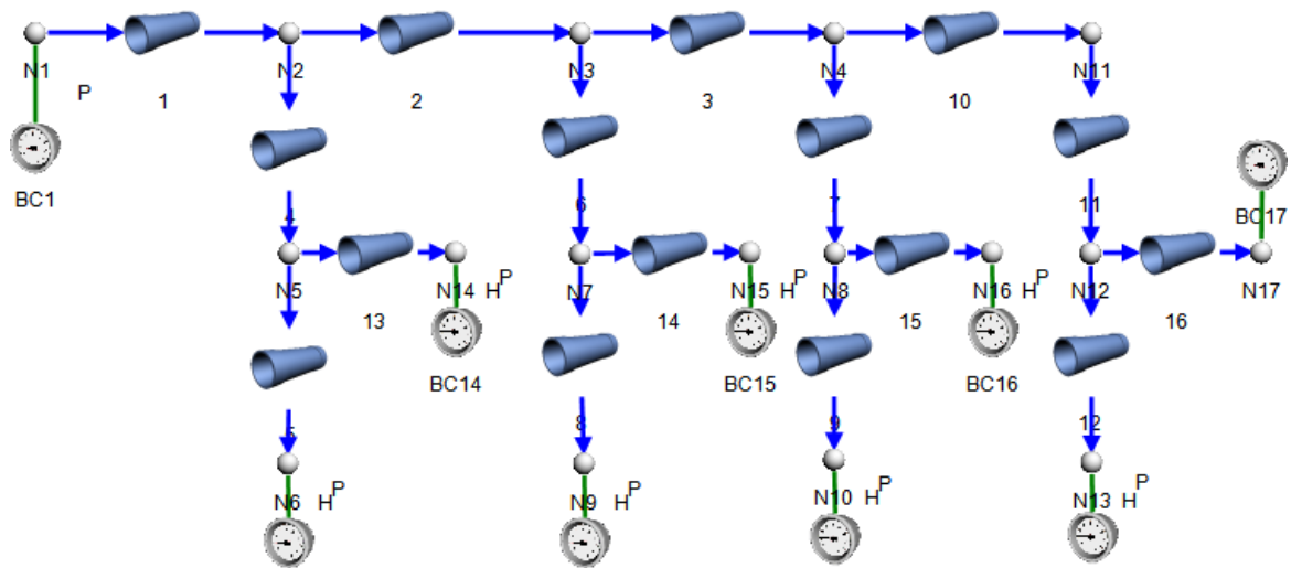
Figure 2: Flownex network of the chilled water distribution system.
