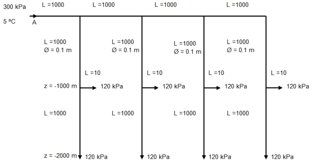
Figure 1: Layout of the chilled water distribution system.
