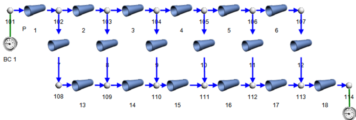
Figure 2: Flownex network.
