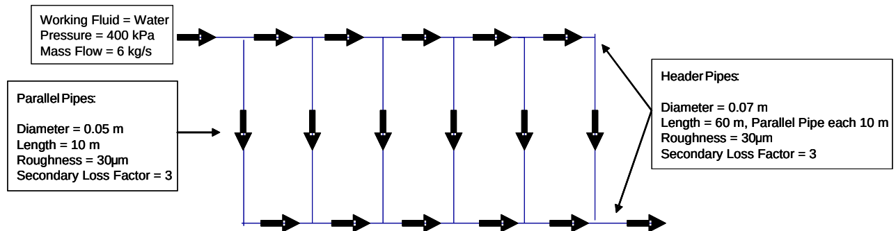
Figure 1: Schematic layout of a water system used to illustrate header flow balancing.
