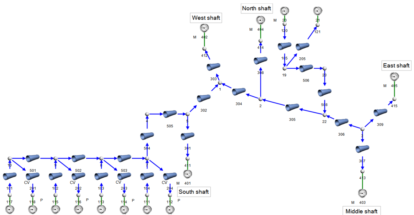
Figure 2: Flownex network of the compressed air network.
