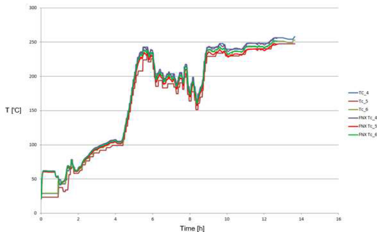
Figure 5: Tube bank inlet temperature comparison
