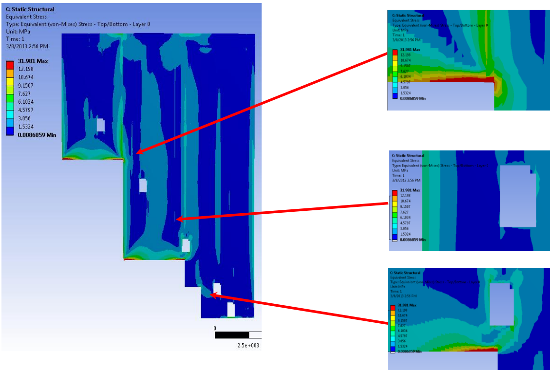
Figure 8: Thermal Stress Results (Tube wall only)
