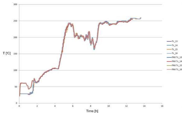
Figure 6: Staith intersection temperature comparison
