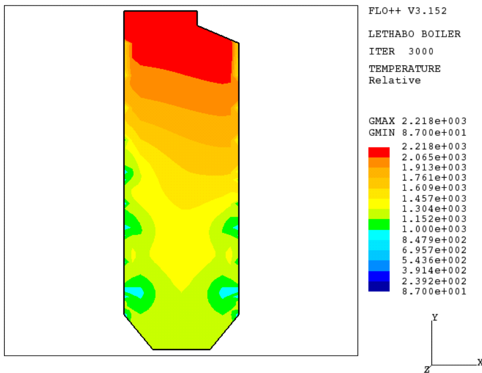
Figure 4: Temperature distribution on burner centreline
